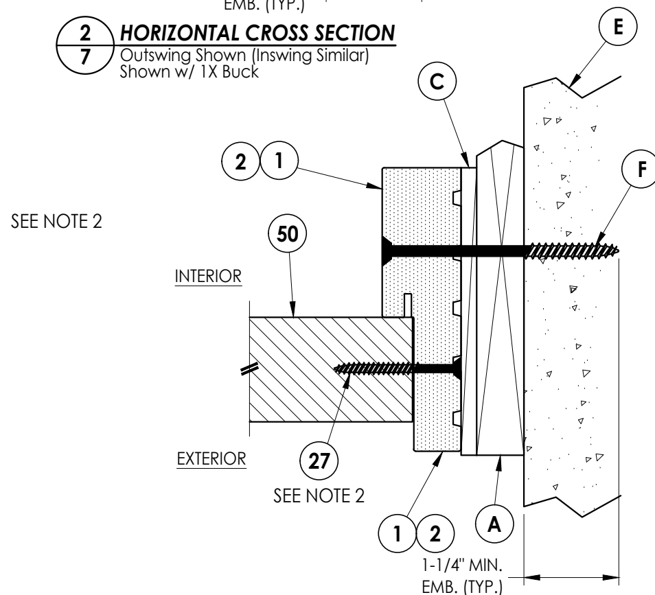
3 HORIZONTAL CROSS SECTION 7 Outswing Shown (Inswing Similar) Shown w/ 1X Buck
