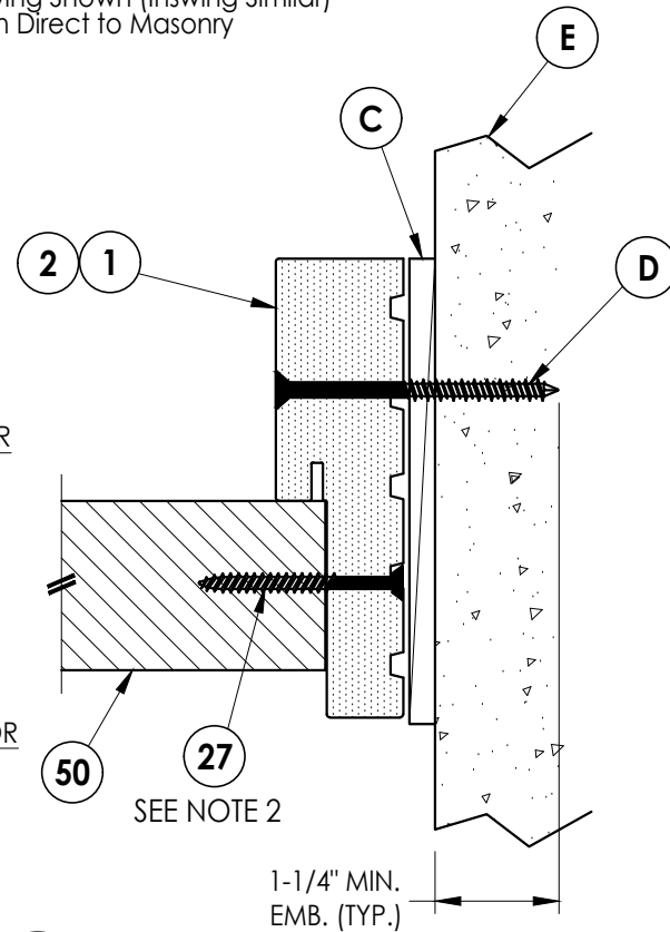
3 8 HORIZONTAL CROSS SECTION Outswing Shown (Inswing Similar) Shown Direct to Masonry
